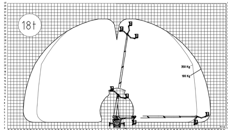
TKA 35 KS working area
